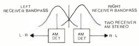
Kahn AM stereo signal can be brought in by two AM mono receivers, one tuned a little high, the other a little low.
